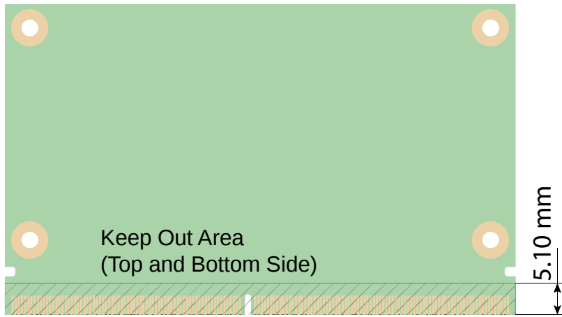
Figure 2: Module Edge Finger Keep Out Area (82mm x 50mm Module)
