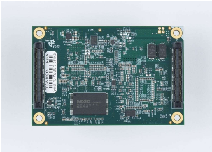
Bottom view showing board-to-board connectors
