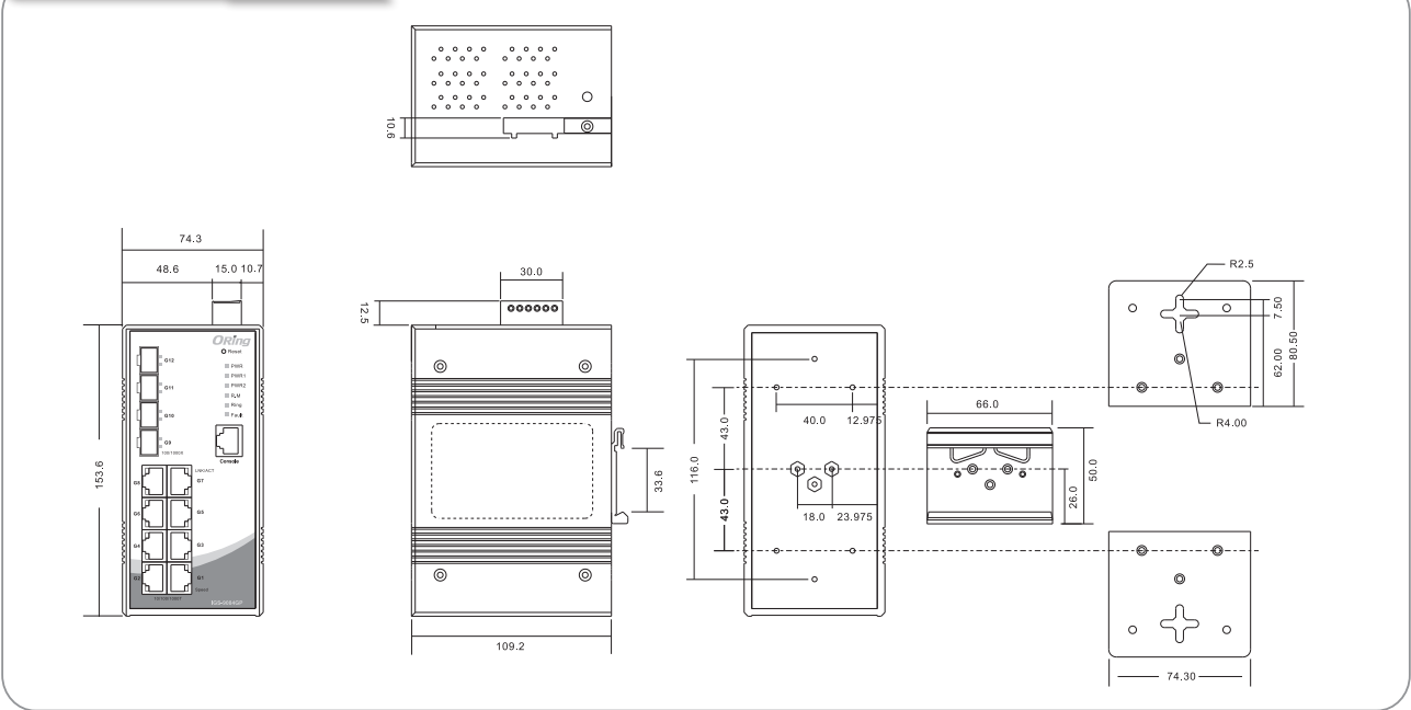
(Unit=mm)
